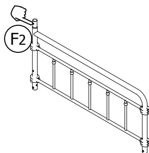
Side Guard Rail T944730 X 1
