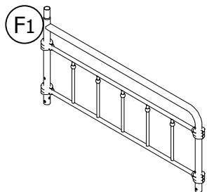
Side Guard Rail T944720 X 1
